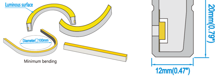
Bending Diagram
