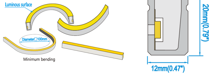
Bending Diagram
