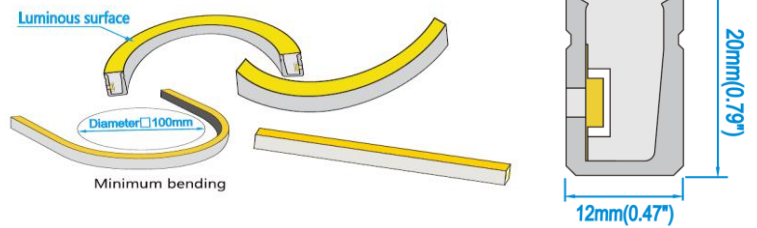
Bending Diagram
